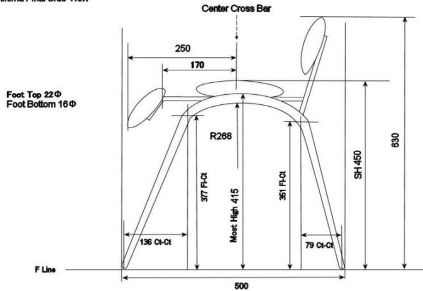
Minima Final Side View
